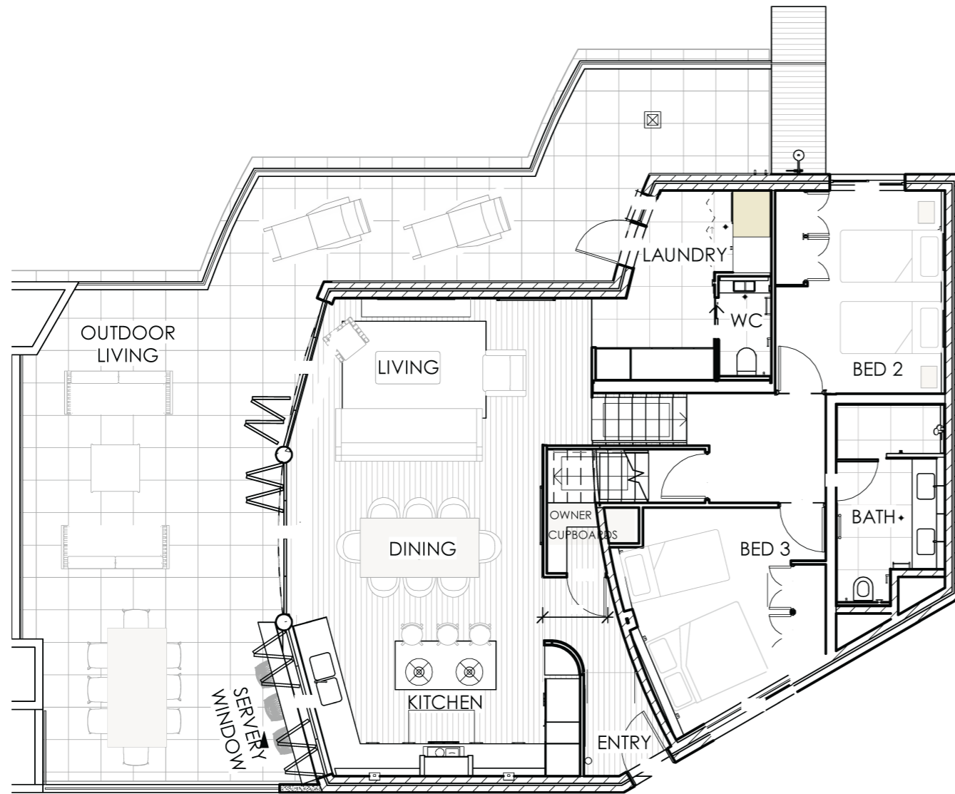
LEVEL 1 + 2 - FLOOR PLAN
