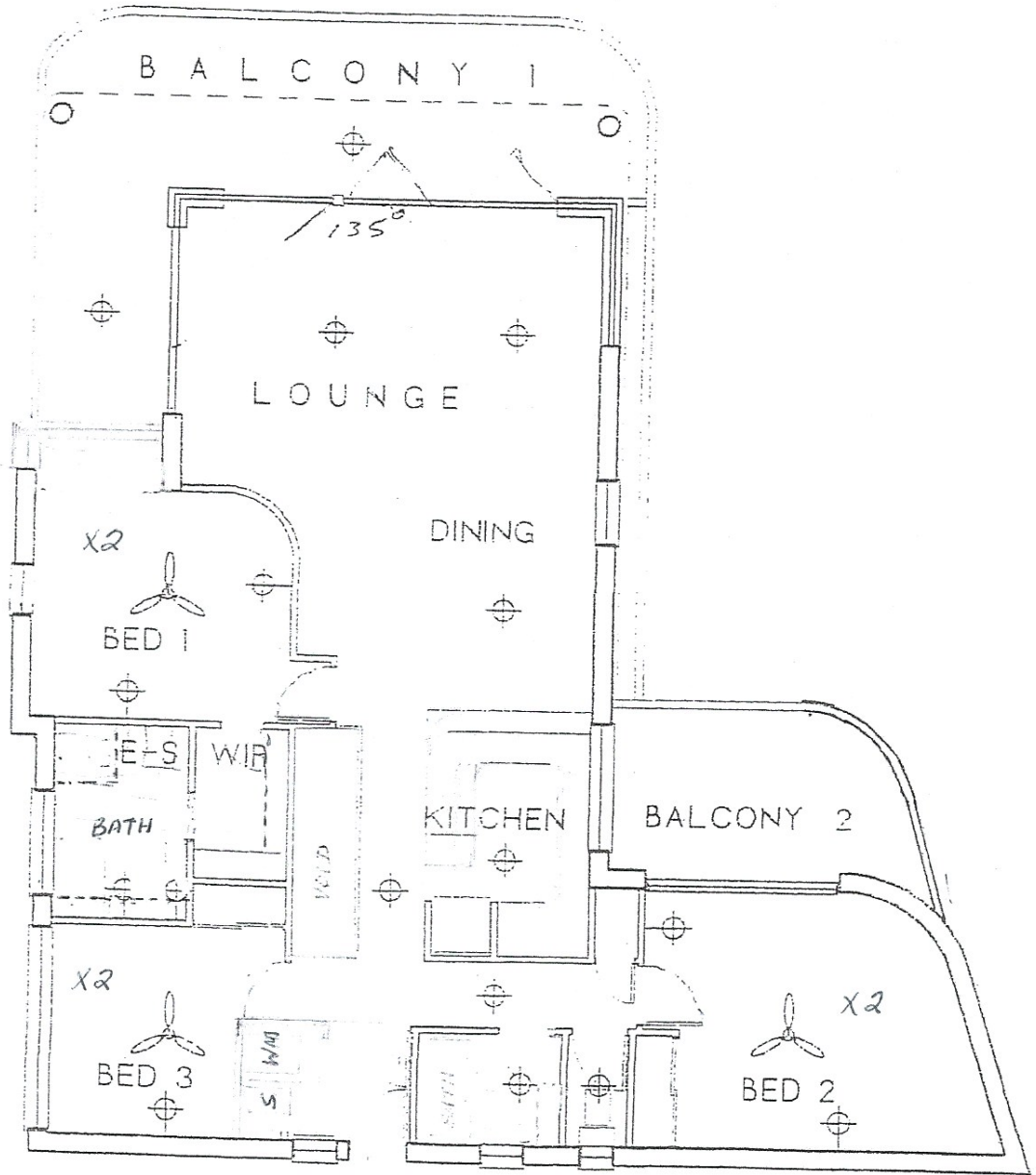
GROUND FLOOR PLAN BAHIA LINDO (UNIT1)
